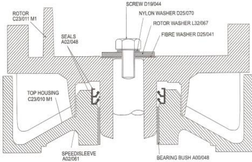
Fig 10: Seal Assembly 1204/1604
